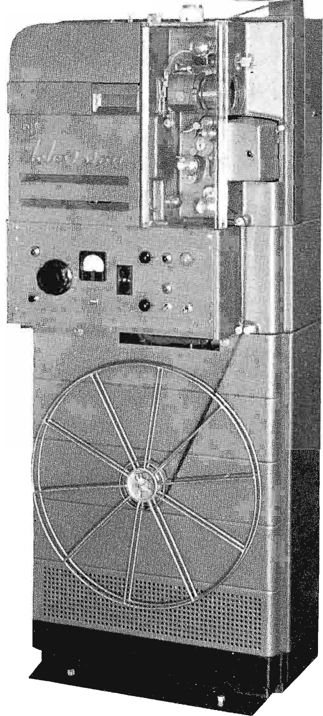
FIG. 1. Cost-saving advantages of the RCA TP-6 Projector include automatic projection lamp change, rapid manual change of sound exciter lamp and simplified maintenance features.
