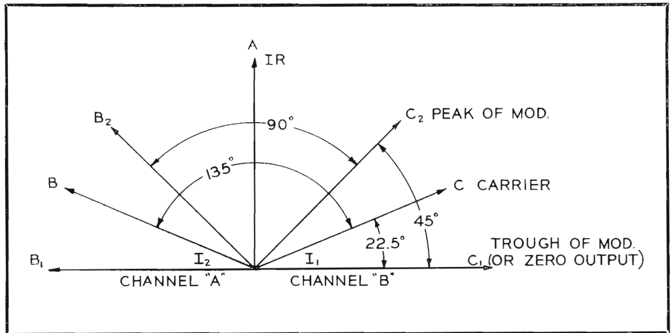
FIG. 6. Ampliphase vector diagram.
