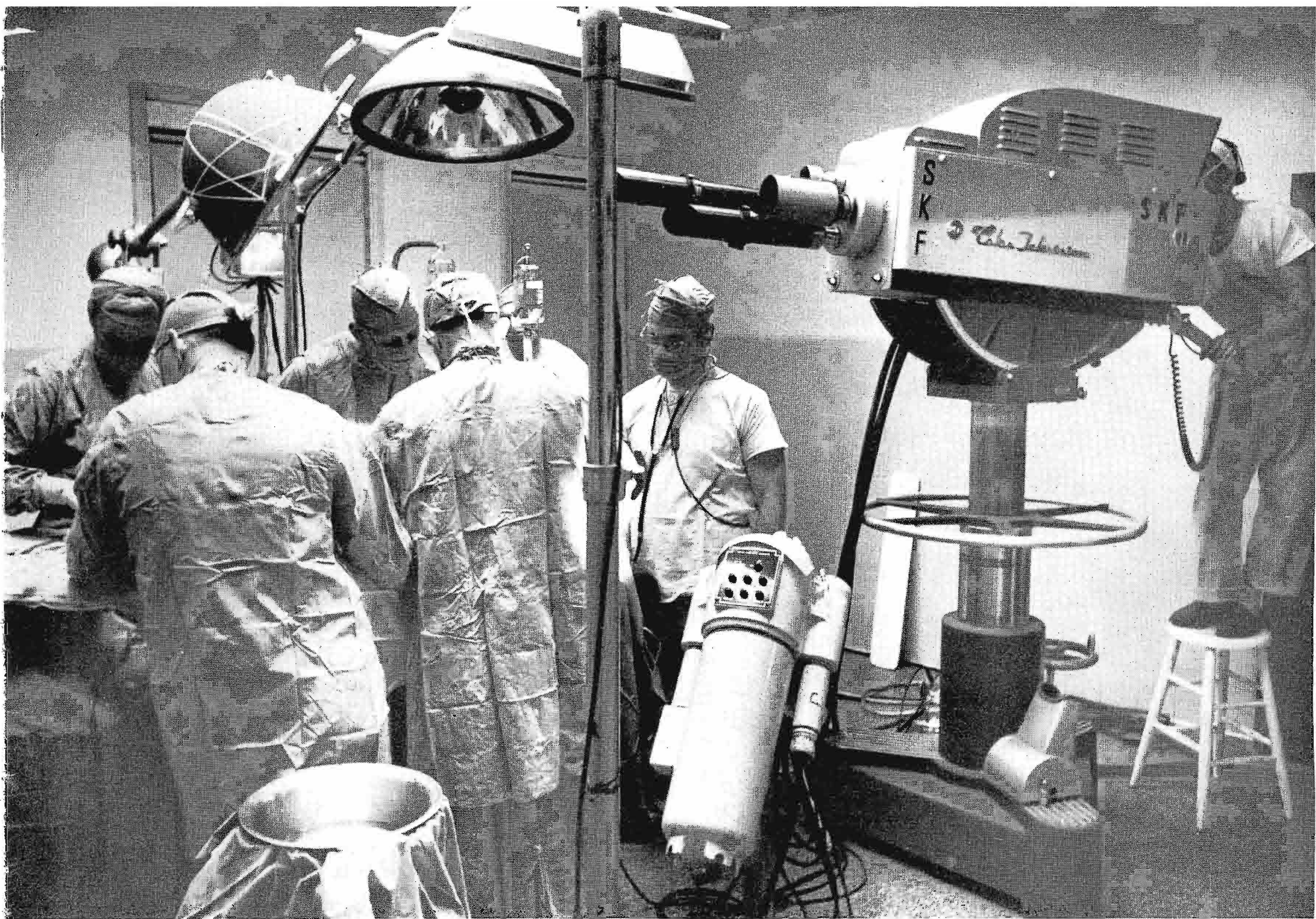
FIG. 2. One TK-41 Color Camera, operated by SKF technician, was used in surgery where a mirror mounted on surgical light fixture at 45 degree angle gave camera an unobstructed view of operating field.
