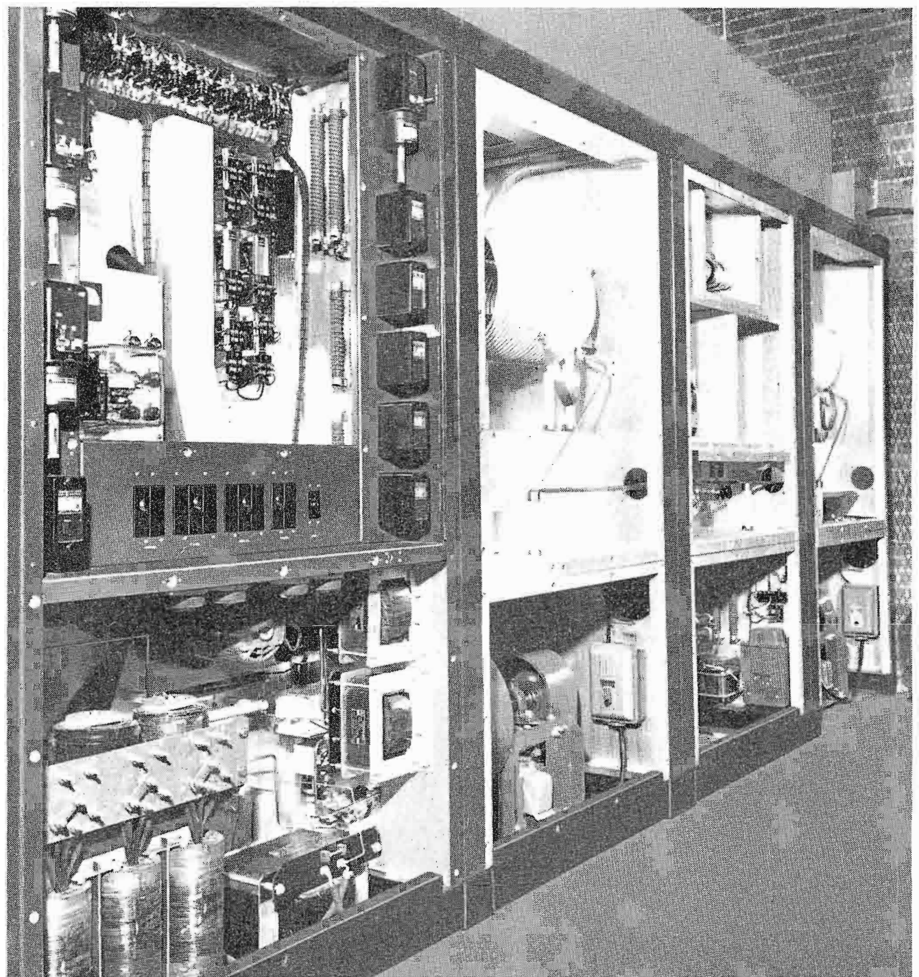
FIG. 3. Rear view of Ampliphase Transmitter showing left to right: a. Rectifier and control. b. Power amplifier. c. Exciter-Modulator and IPA. d. Power amplifier.
