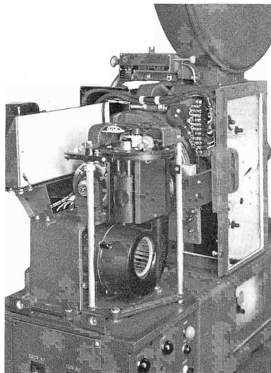
FIG. 9. Automatic lamp change mechanism of the TP-35. Spare lamp instantaneously moves into place should "run" lamp fail.
