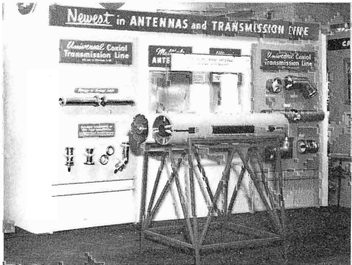
FIG. 11. Antenna and transmission line display included Traveling Wave Antenna for high-band VHF operations as well as 3/8 and 6/8-inch Universal Transmission Line for use on channels 2 through 83.
