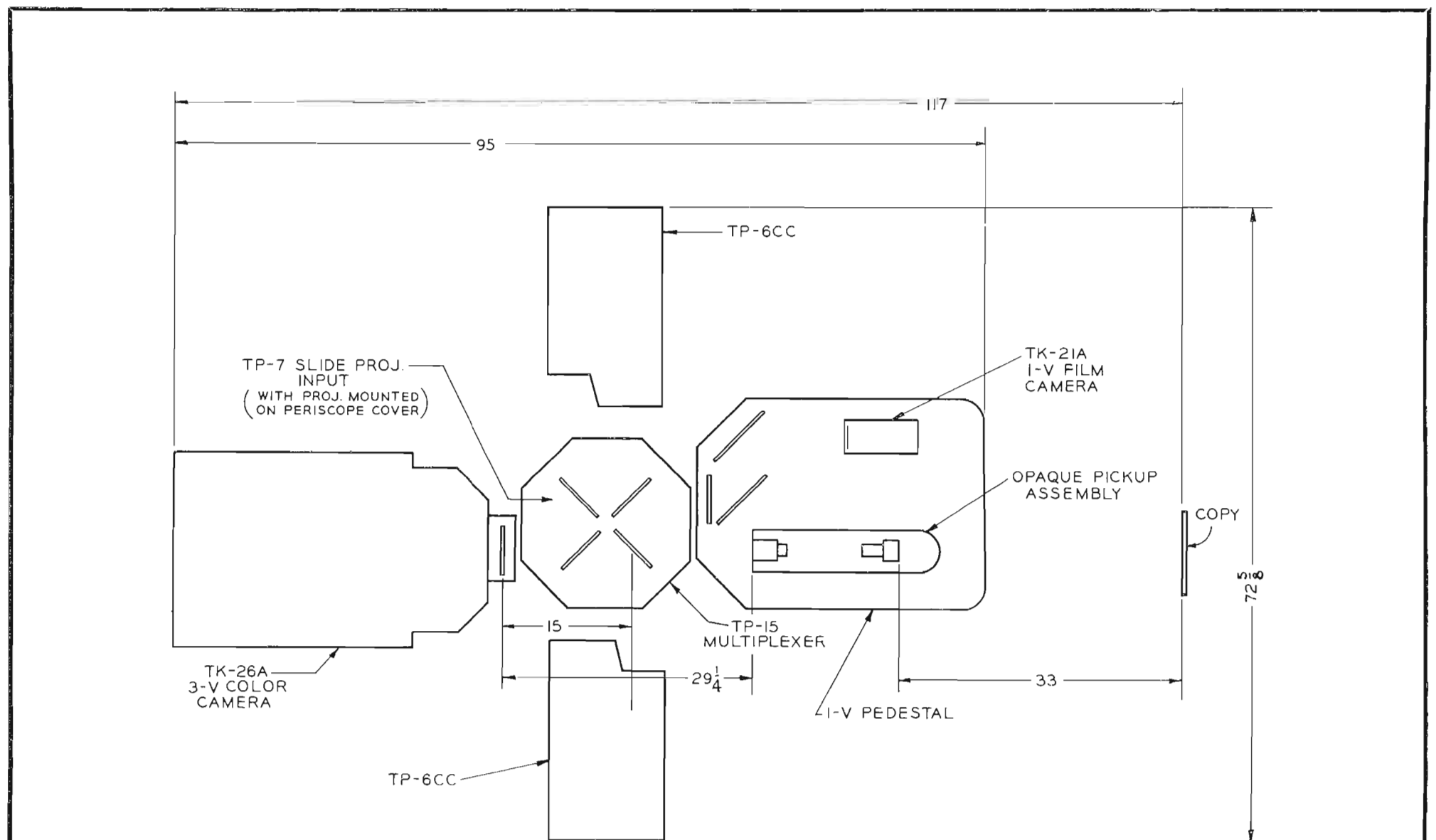
FIG. 13. Layout of professional film system for monochrome or color operation. Basic system for monochrome only is represented by the same layout, omitting the TK-26A 3-V Color Camera (left).
