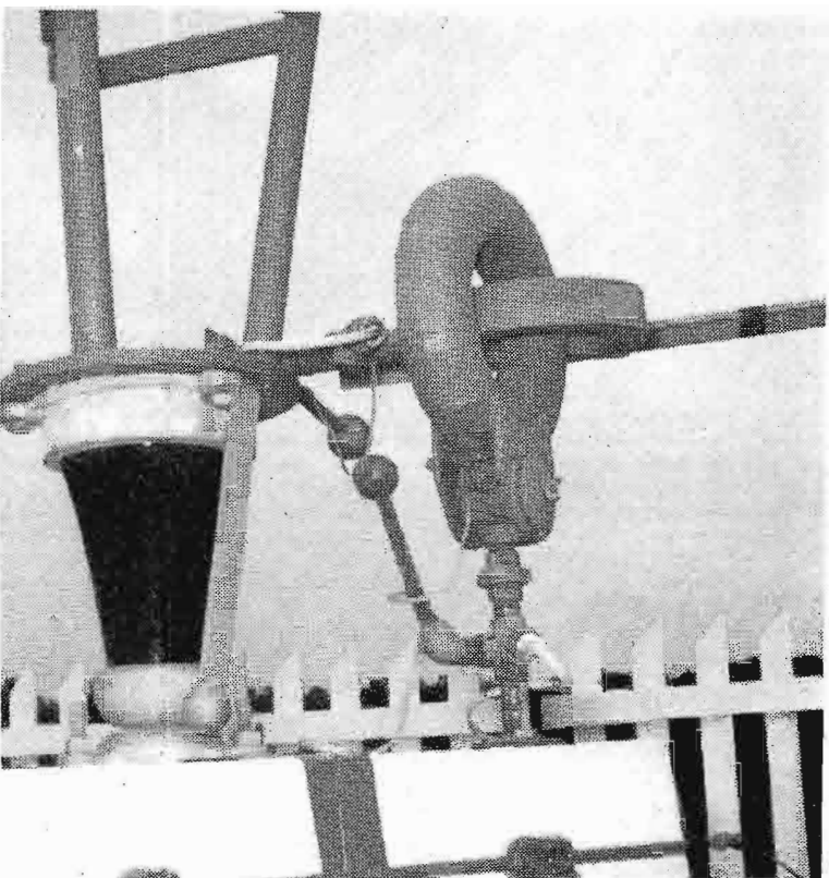
FIG. 14. Typical installation of Austin lighting transformer to isolate ac lighting circuit from rf.
