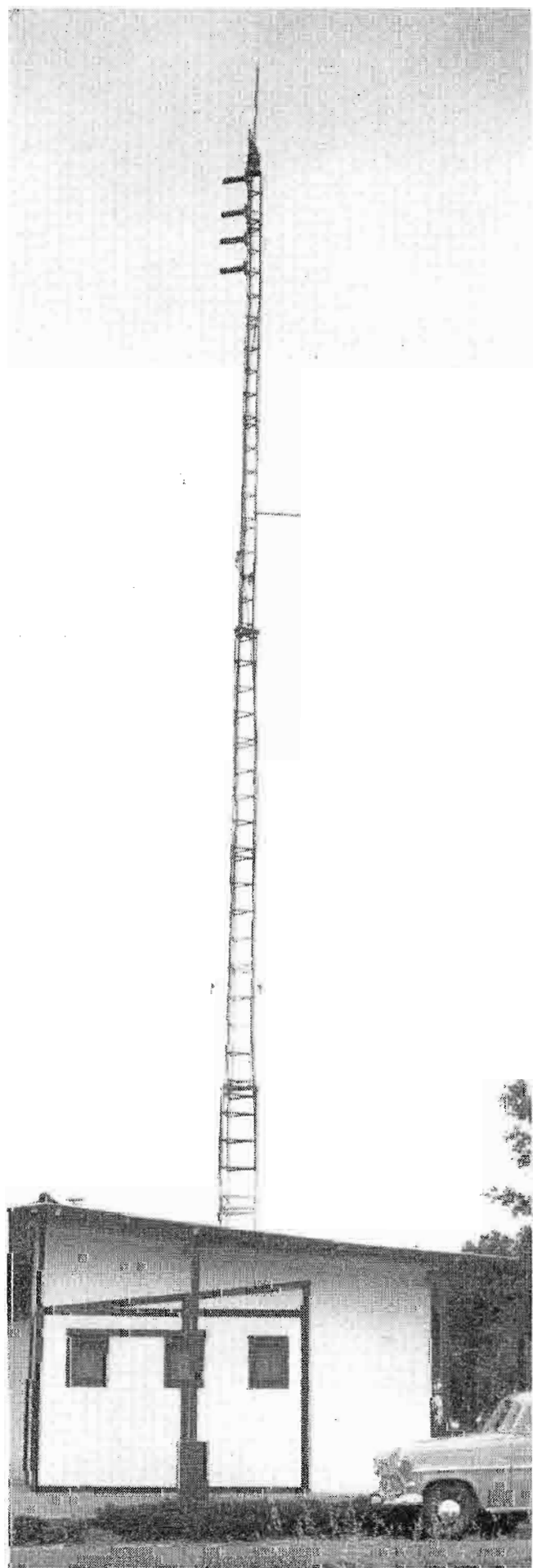
FIG. 31. Transmission antennas at Maxoqueira: (Top) 32 mc whip for two-way radio communication with Lisbon and Gloria. (Directly beneath top) Four helix antennas to send received programs to Lisbon studios. (Center) 90 mc dipole reflector for keying three-kw cue transmitter (at Gloria) for CW communications with Holzkirchen.
