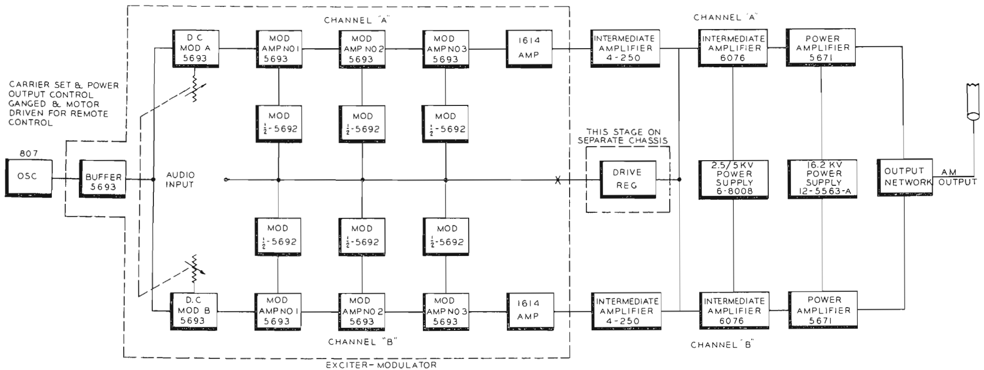
FIG. 2. Basic circuits of RCA Ampliphase Transmitter.
