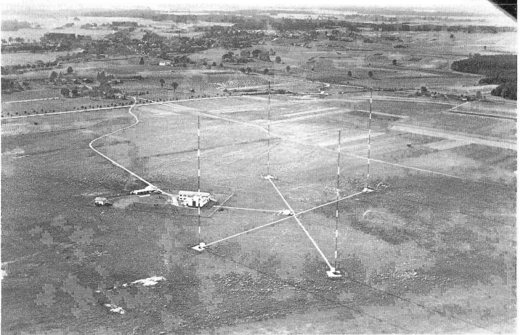
FIG. 27. RFE relay station at Holzkirchen, Germany. This is used as a program link with RFE transmitters in Portugal.
