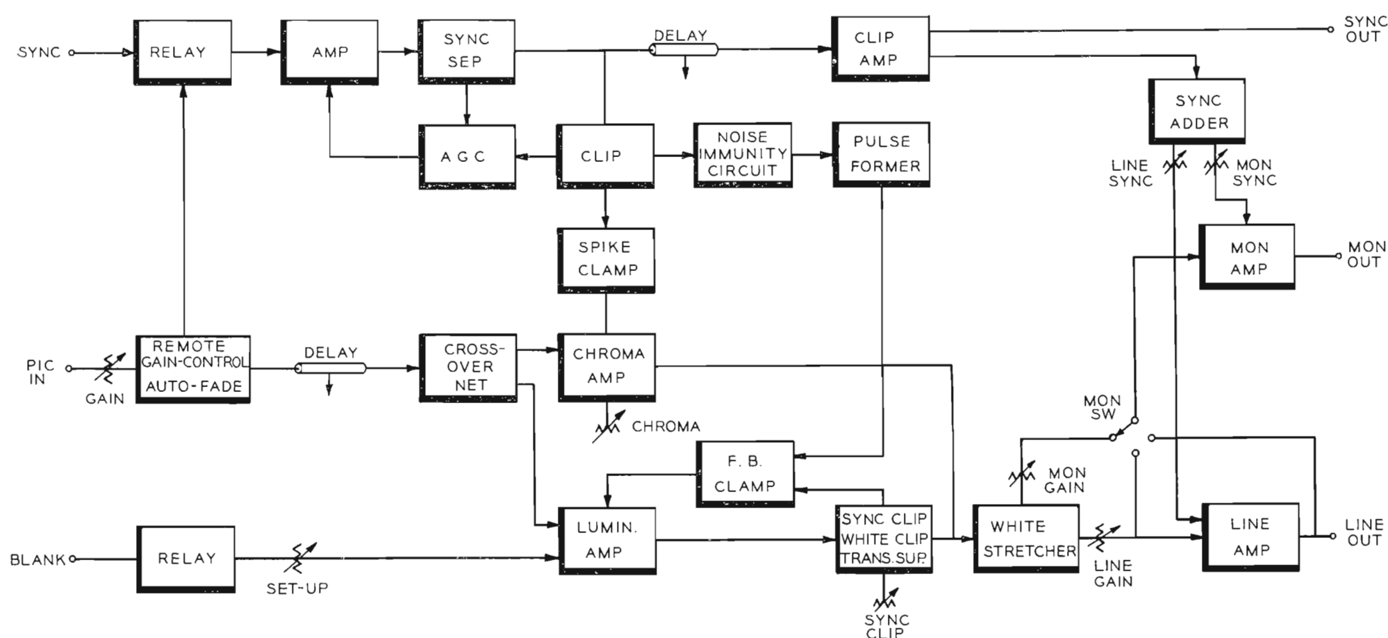
FIG. 2. Simplified block diagram of TA-9 Stabilizing Amplifier. The composite picture signal traverses three paths; chrominance, luminance and sync.
