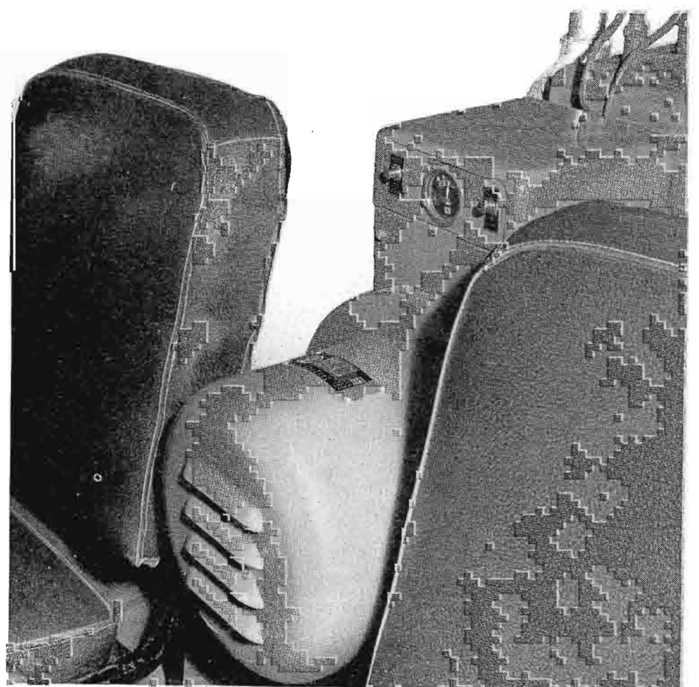
FIG. 7. Because of the size of power plant it was necessary to let generator extend between seats of jeep.
