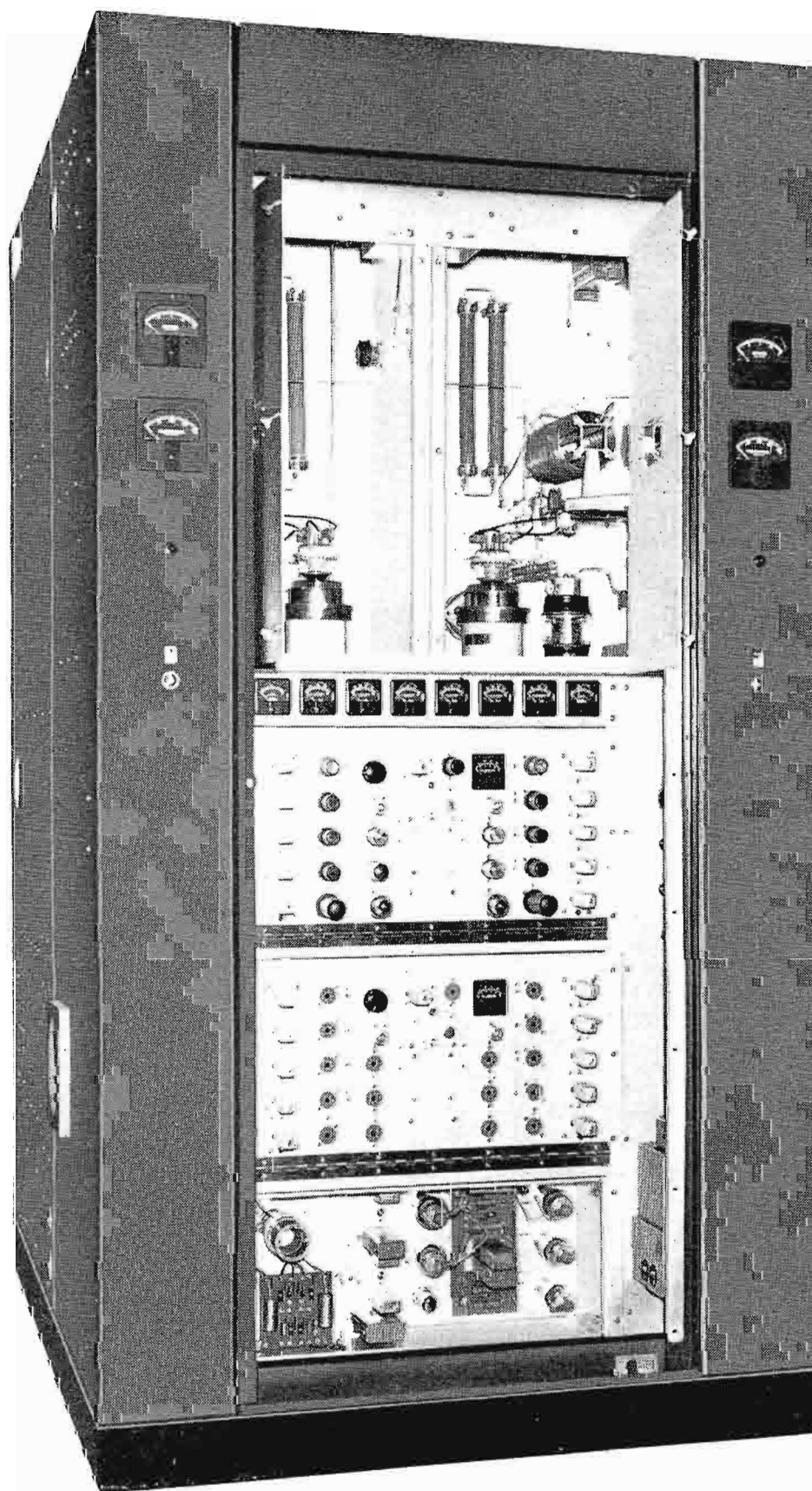
FIG. 5. Front view of Exciter-Modulator cubicle showing use of two E-M units. At extreme bottom is drive regulator (right) and feedback rectifier assembly (left). At the top are first and second IPA stages.
