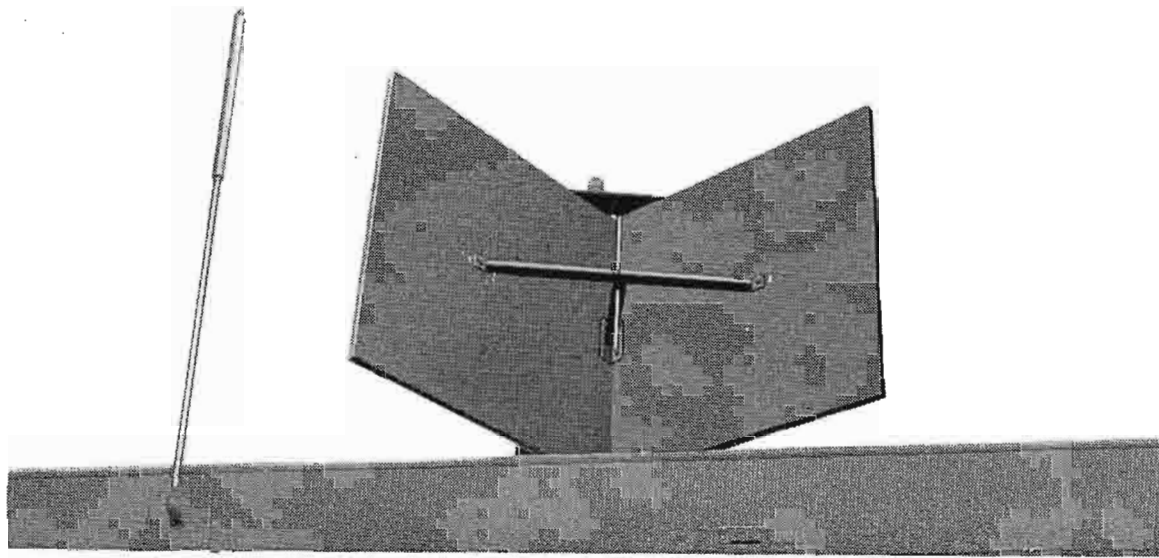
FIG. 4. Close-up of coax and corner reflector antennas atop mobile unit. These are used for 450 mc transmission to WHHM studios.
