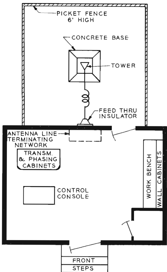
FIG. 3. Plan view combination antenna tuning and transmitter building.
