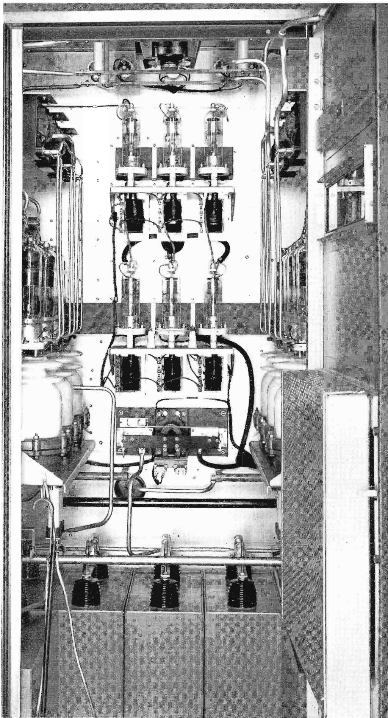
FIG. 13. Front view rectifier and control cubicle.
