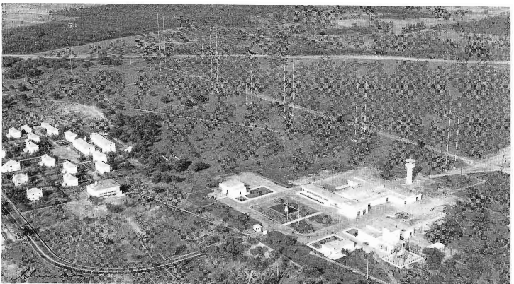
FIG. 38. Transmitting plant at Gloria, Portugal. Note housing facilities for personnel at left. Part of antenna system can also be seen.
