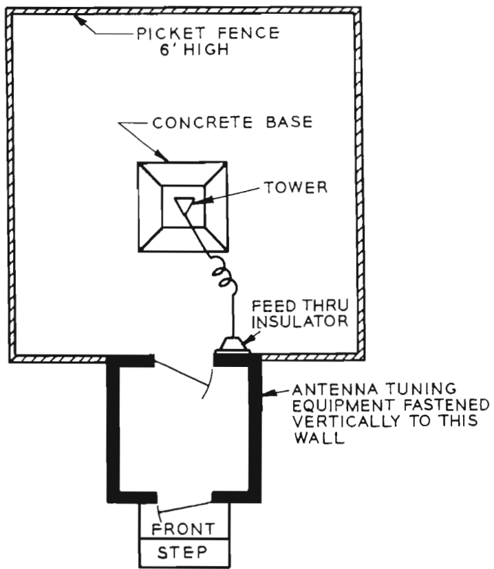
FIG. 2. Plan view of the antenna tuning house.
