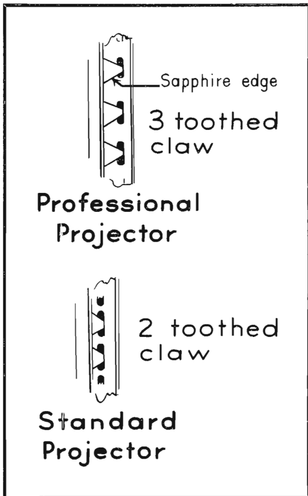
FIG. 2. Comparison of three-tooth vs. two-tooth claw pull-down.
