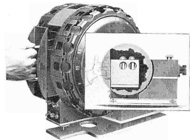
FIG. 11. Quick lamp change feature of the TP-7. Spare lamp can immediately be moved into place by pulling handle as shown.
