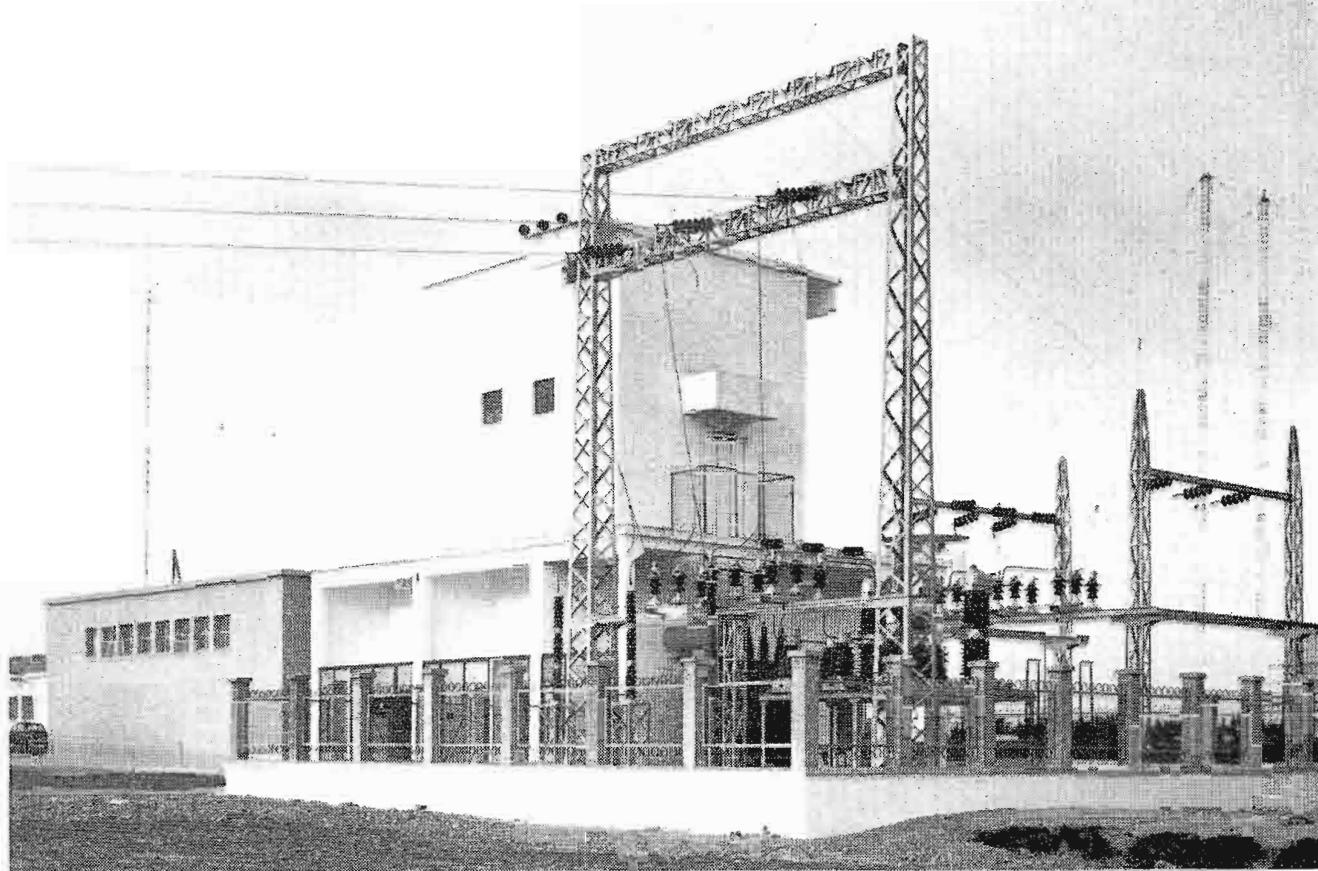
FIG. 46. Main power substation at Gloria.
