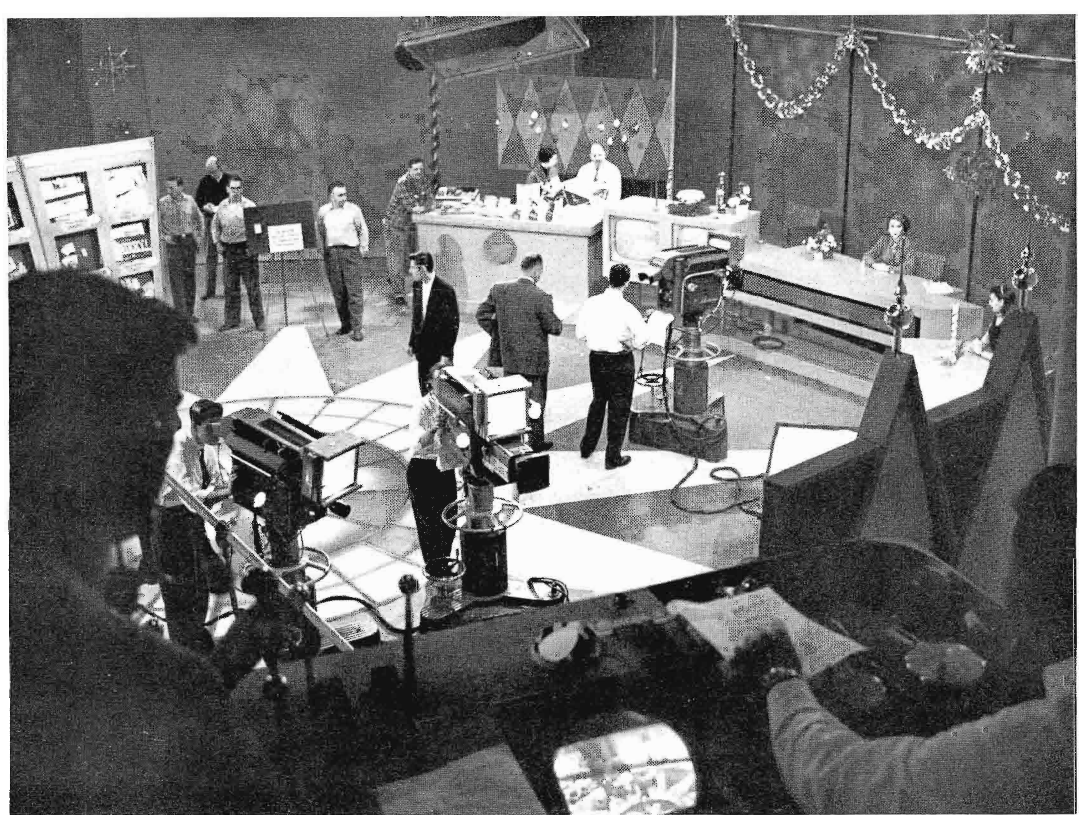
THE COMMERCIAL STUDIO. The space control area would serve to the maximum the requirements of the Commercial Studio. The closest approach yet made to this kind of presentation is in use in New York City at the NBC 'Home' studio, designed by the author. Here the emphasis is placed on the ability to handle 'things' expertly. One hour of air time is televised each day with only six hours of 'in studio' preparation time.
