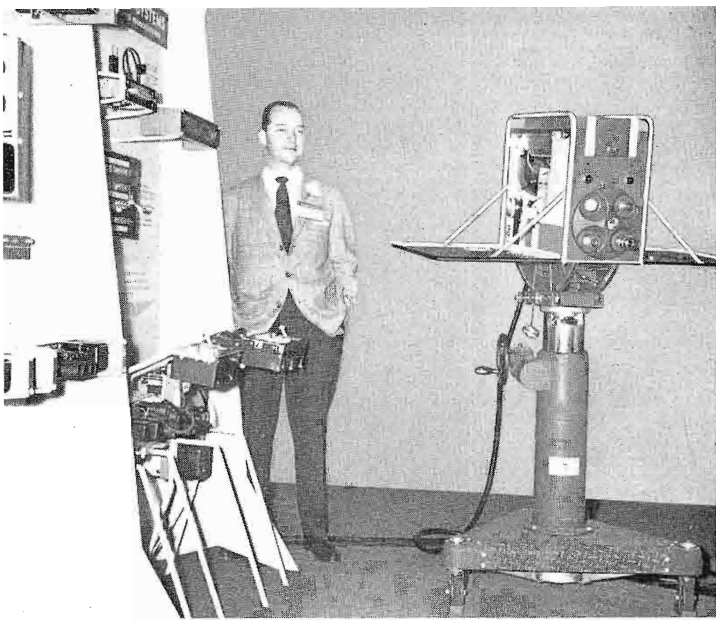
FIG. 3. RCA TK-15 Vidicon Studio Camera and friend both view the tropical scene. This new camera, built to broadcast standards, was shown in operation for the first time.
