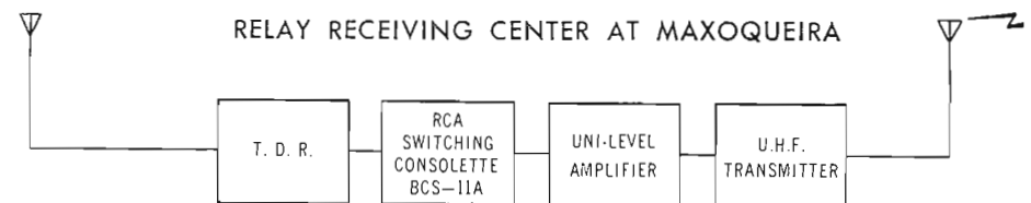
FIG. 29. Block diagram showing operations in Portugal at three geographic locations.
