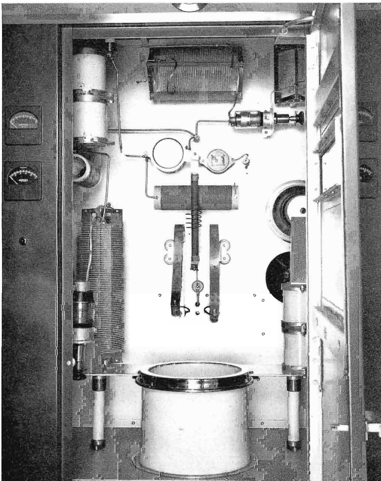
FIG. 9. Front view of PA cubicle.
