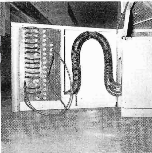
FIG. 42. Provision for patching R-F sample of any transmitter for test purposes, located at one end of transmitter control console.
