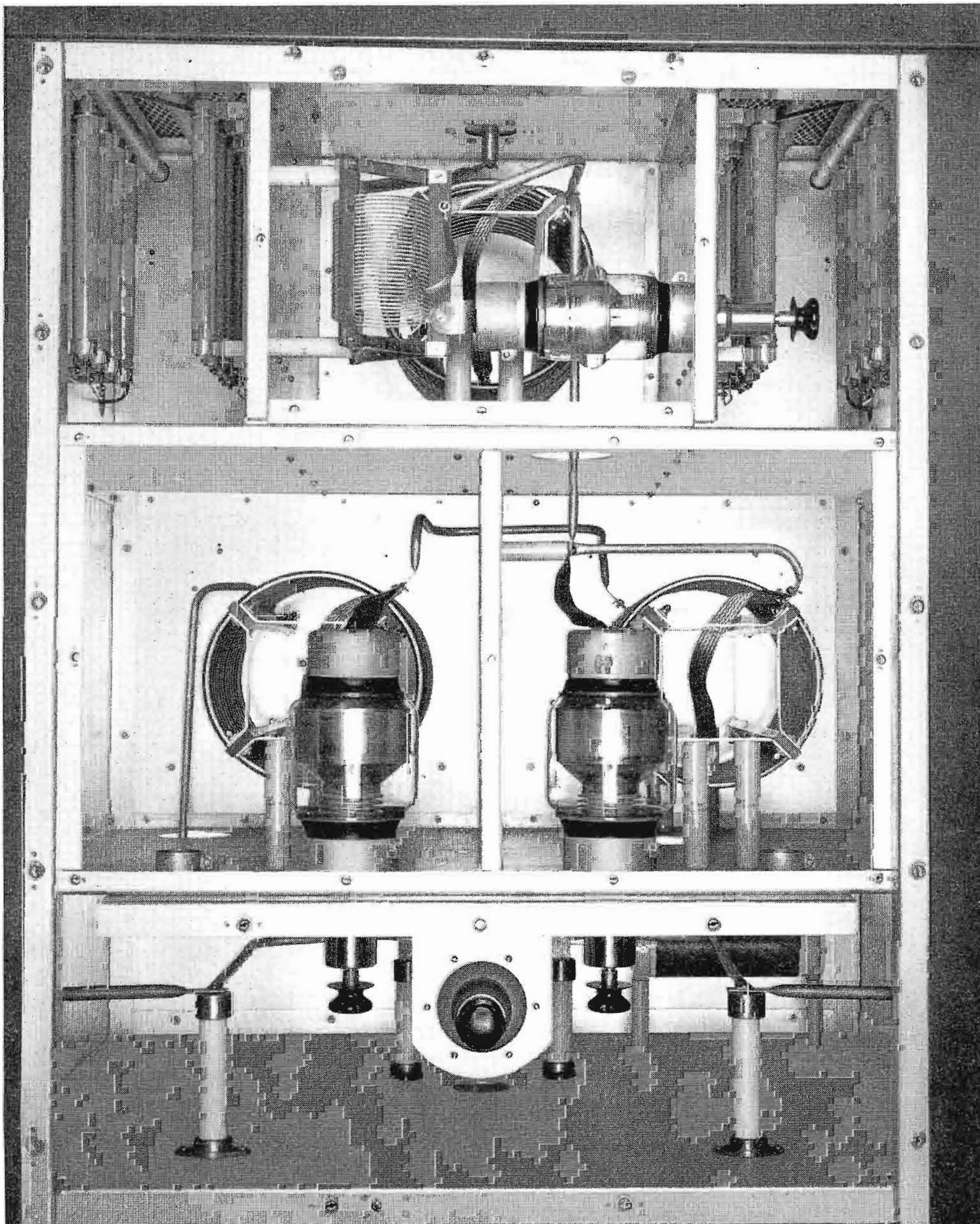
FIG. 11. Rear view of Exciter-Modulator cubicle showing combining network and harmonic filter components.
