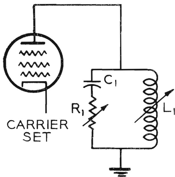
FIG. 7. Adjustable Phase Shifter.
