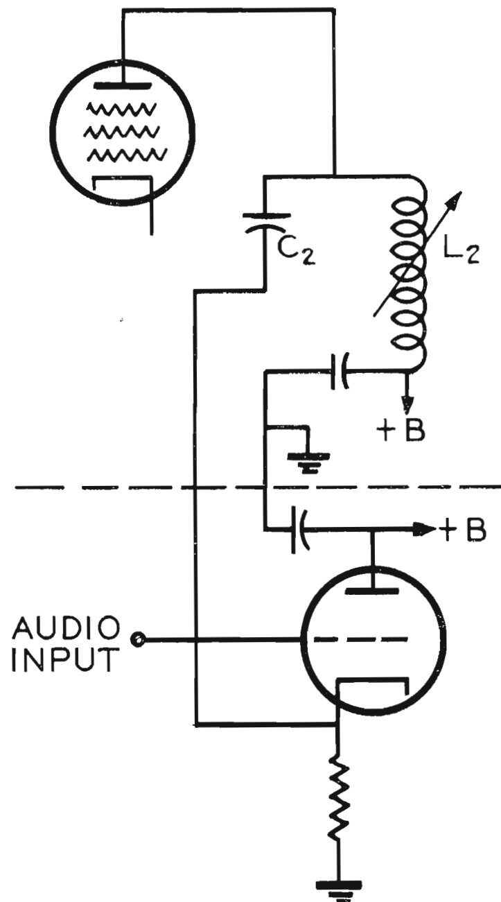
FIG. 8. Modulated Amplifier and Modulator.
