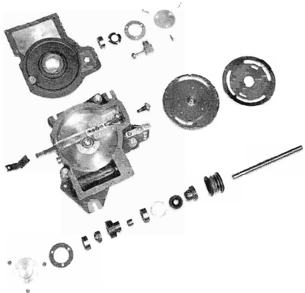
FIG. 3. Exploded view of the intermittent mechanism which permits claw to move straight up and down, engaging the film to its maximum extent.
