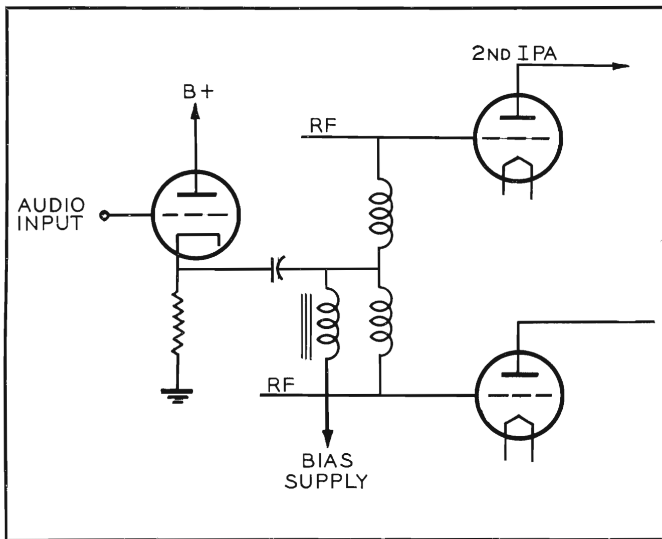
FIG. 12. Simplified circuit of Drive Regulator.
