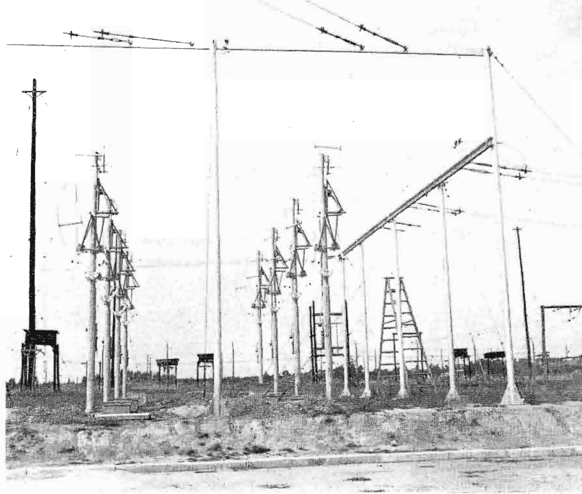
FIG. 51. Typical antenna switching group that handles two transmitters and four antennas.
