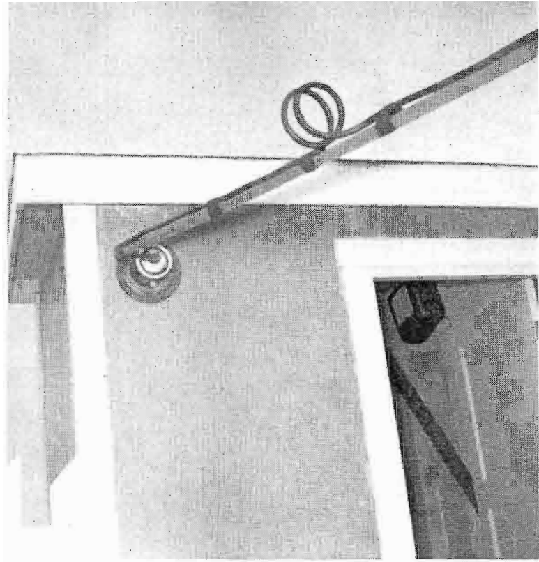
FIG. 12. Note two-turn coil formed in the antenna feed line to retard lightning.
