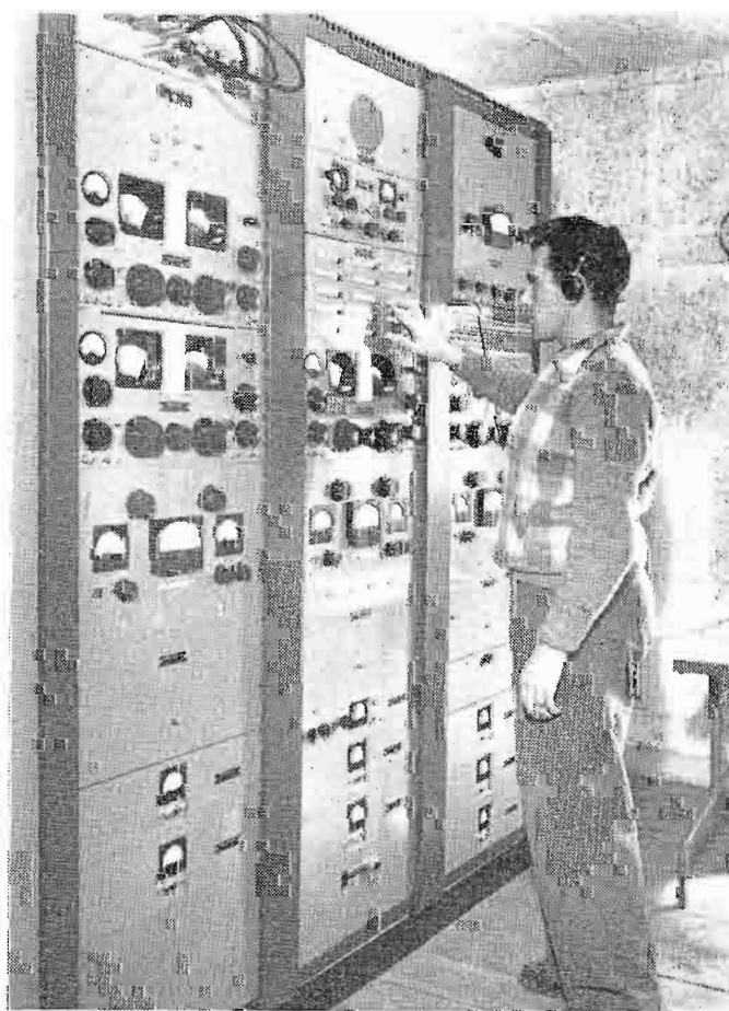
FIG. 32. Audio control at Maxoqueira handles incoming program circuits from Germany.
