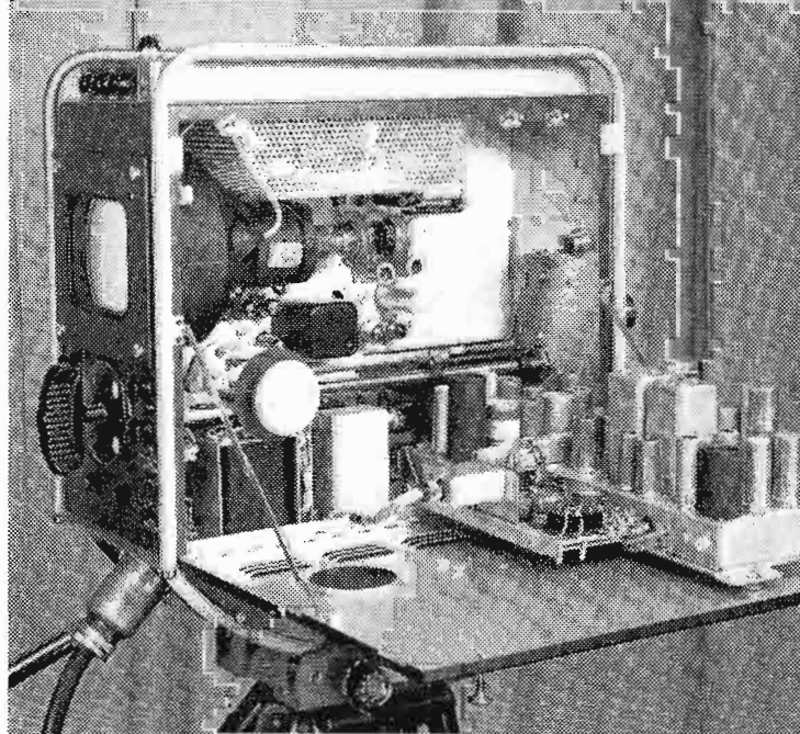
VERTICAL CHASSIS CONSTRUCTION
