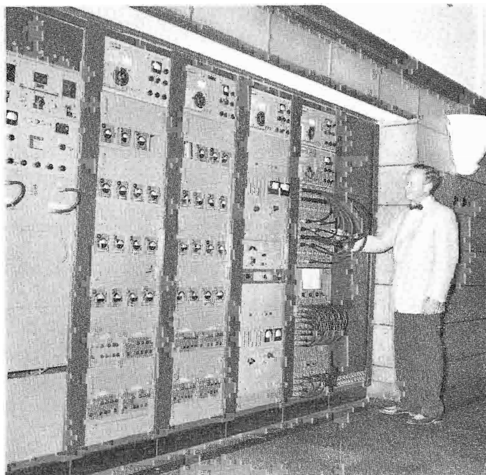
FIG. 48. Meredith L. Koerner, Technical Director, at centralized oscillator control panel.
