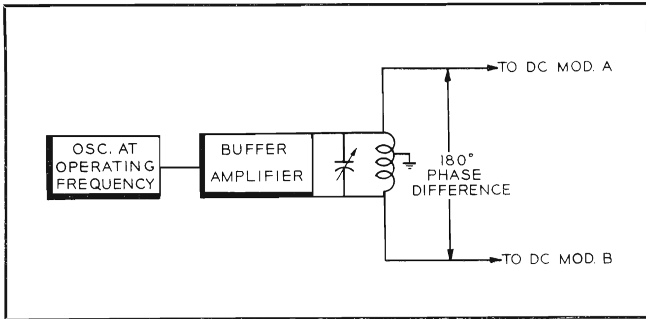
FIG. 4. Exciter-Modulator circuit.
