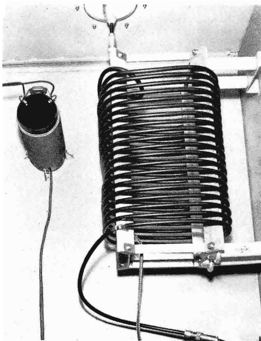
FIG. 13. Use of lighting choke to isolate ac and rf. (Note this is mounted at left of isolation coil in typical installation in weather-proof cabinet shown above.)
