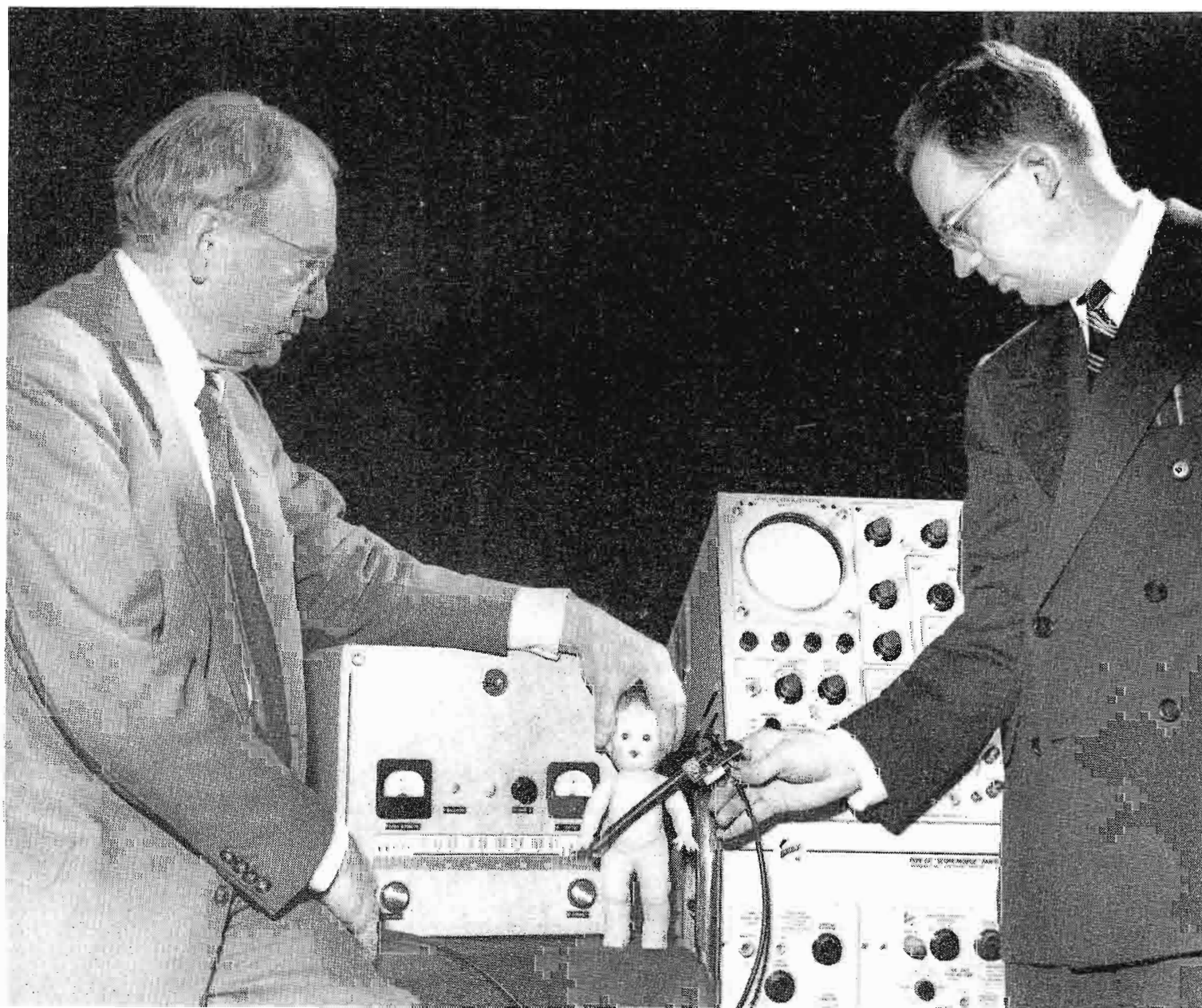
FIG. 3. Output of the "Radio Pill" is picked up by ferrite loop antenna held close to the body (doll in illustration). The antenna is connected to an FM receiver, and the output of the receiver is being fed to an oscilloscope. (The output could be fed to a recording galvanometer for making a permanent record.) The doctor can then observe the trace and diagnose the illness.
