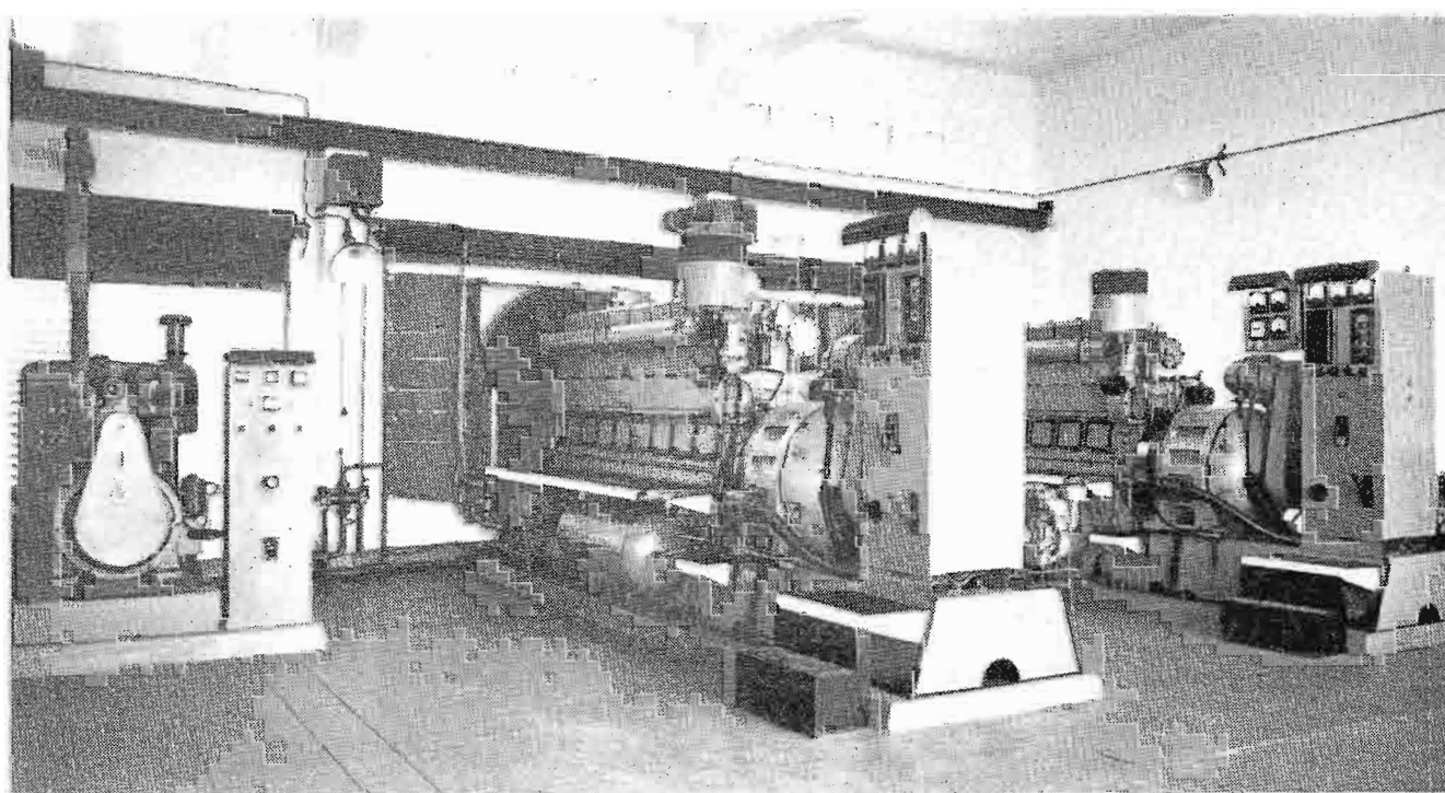
FIG. 47. Emergency power supply at Gloria.
